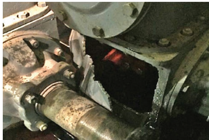
Figure 6: Busbar chamber, showing fault damage (photo: courtesy of Electricity North West)
