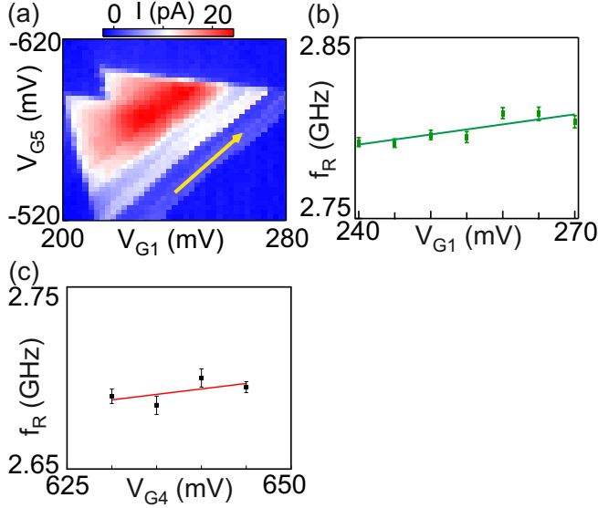
FIG. S5. (a) Current of the blockade transition as a function of V_{G1} and V_{G5} with V_{SD} = 8 mV and V_b = -210 mV. (b) The dependence of f_R on gate voltage along the yellow arrow. (c) Resonance frequency measured with different voltage applied to V_{G4} , when B_z fixed at 0.079 T.
