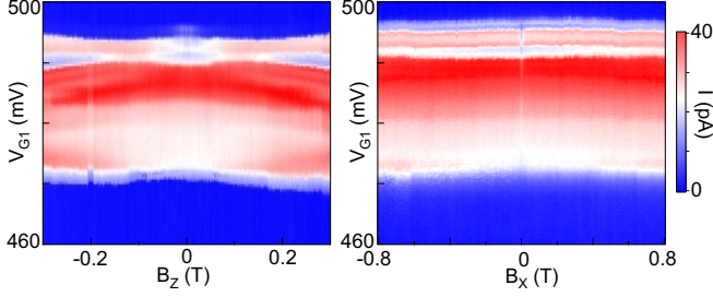
FIG. S3. Current at a blocked transition as a function of V_{G1} along the detuning axis and of magnetic field. In longitudinal magnetic field (a), the current shows a zero-field peak due to hyperfine mixing; in transverse field (b) there is a zero-field dip and a sustained B_x -independent current for finite B_x , consistent with the presence of different valley-mixing phases in the two dots.
