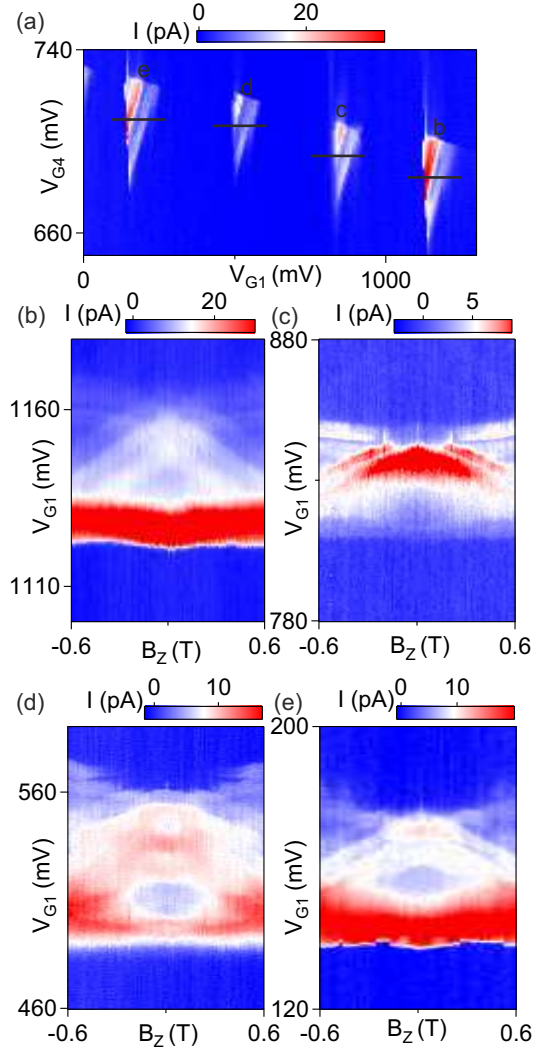
FIG. S2. (a) Current as a function of V_{G1} and V_{G4} with V_{SD} = 10 mV, for a different gate setting from that of Fig. 1. The four marked bias triangles correspond to four successive hole transitions of the left quantum dot in the p-n regime. (b)-(e) Current as a function of V_{G1} and B_z , measured along the black lines marked in panel (a). The lower edges track the ground-state energy of the left dot.
