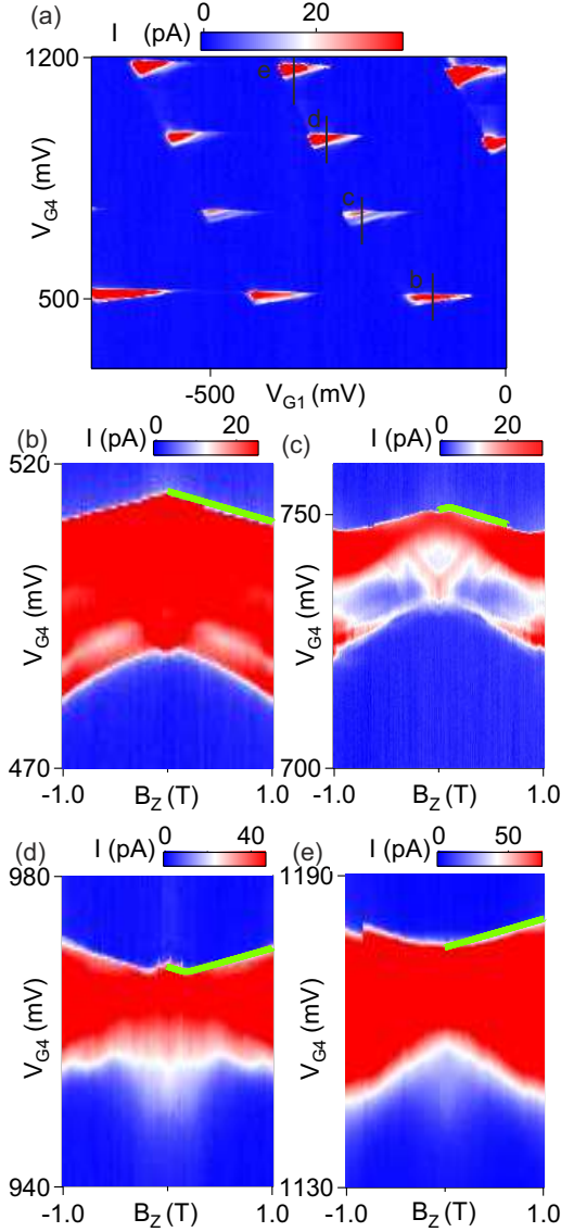
FIG. S1. (a) Current as a function of V_{G1} and V_{G4} with V_{SD} = 10 mV, for a slightly different gate setting to Fig. 1. The four marked bias triangles correspond to the first four electron transitions of the right quantum dot in the p-n regime. (b)-(e) Current as a function of V_{G4} and B_z , measured along the black lines marked in panel (a). Green lines run parallel to each upper edge, which maps out the ground-state energy of the right dot.
