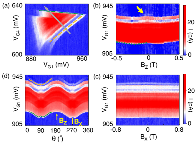
FIG. 2. (a) Current at a Pauli-blocked transition, with V_{\text{SD}} = 8 \text{ mV} , V_{G2} = V_{G3} = -210 \text{ mV} , \mathbf{B} = 0 . Dashed (dotted) line marks ground-state degeneracy between left and right dots (between right dot and lead). Arrow marks detuning axis. (b) Current as a function of V_{G1} along the detuning axis and of the magnetic field parallel to the nanotube. Arrow marks a region of the Pauli blockade leakage current near zero field. (c) As (b) for perpendicular field. (d) As a function of the field angle for |\mathbf{B}| = 0.8 \text{ T} . Color scales in (a),(d) match (c). Dashed and dotted curves highlight the same transitions as in (a).
