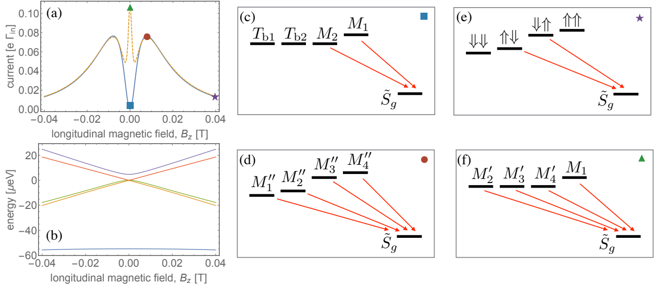
FIG. S4. Leakage current, energy spectrum, and inelastic downhill interdot tunneling processes in a longitudinal magnetic field. (a) Simulated leakage current as a function of magnetic field without (solid line, E_N = 0 ) and with (dashed line, E_N = 0.16 \mu\text{eV} ) hyperfine interaction. Other parameters: t = 3 \mu\text{eV} , t_{\text{spin}} = 11 \mu\text{eV} , \varepsilon = 50 \mu\text{eV} , g_L = 2 , g_R = 17 ; number of nuclear-field realizations: 5000. (b) Energy eigenvalues of the tunnel-coupled (1,1)-(0,2) states as functions of the longitudinal magnetic field B_Z . Parameters as in (a) with E_N = 0 . (c,d,e,f) Energy levels (black horizontal lines) and inelastic, energetically downhill interdot tunneling processes (red arrows) for the parameters marked in (a).
