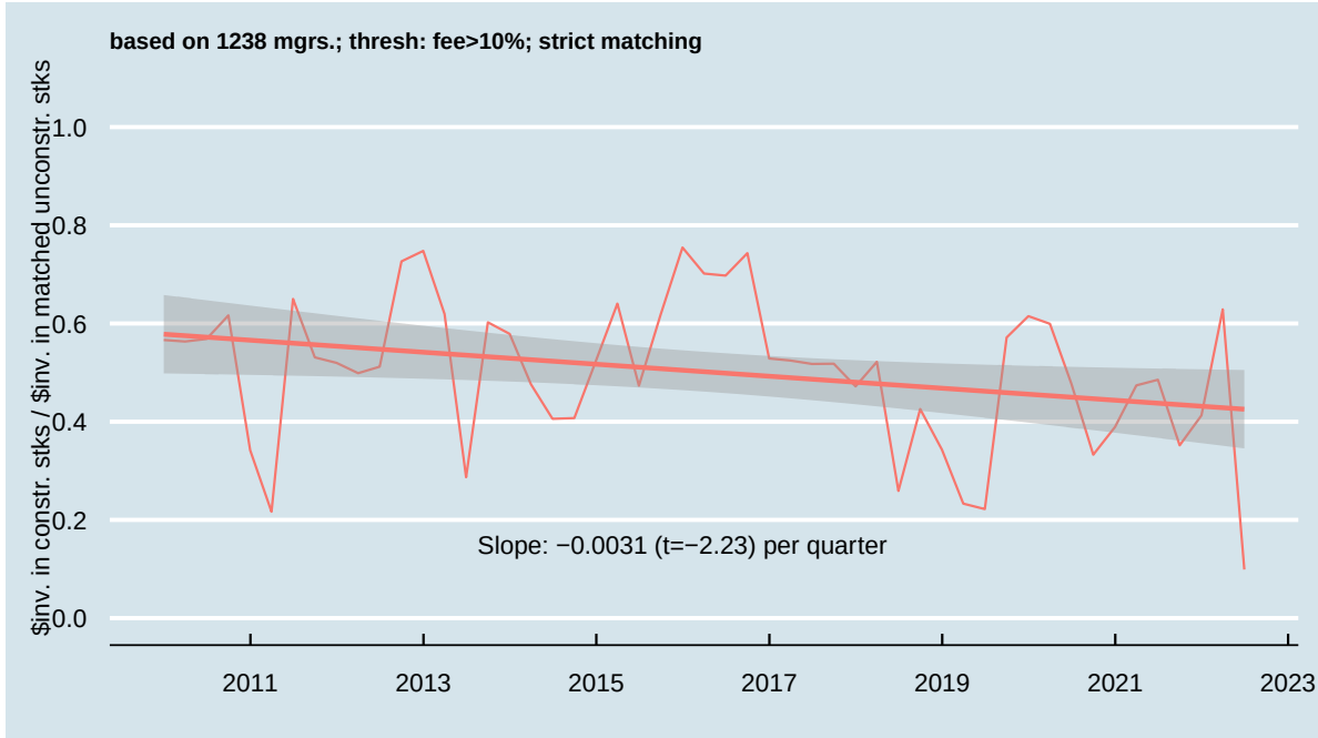
Figure 13: Ratio of investment in constrained vs. matched unconstrained stocks
