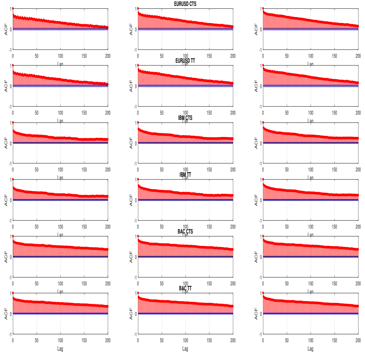
Figure C.2: ACF of the log-transformation of the negative estimates of daily quantiles, \hat{q}_{p,d} , computed from scaling up estimates of intraday quantiles estimated from data sampled in TTS and CTS (use the DMA estimator of Hurst coefficient and the frequency of 5 minute to sample the data). The first column corresponds to p = 1\% , the second column corresponds to p = 2.5\% and the third column corresponds to p = 5\% . The blue line represents the 95% confidence interval.
