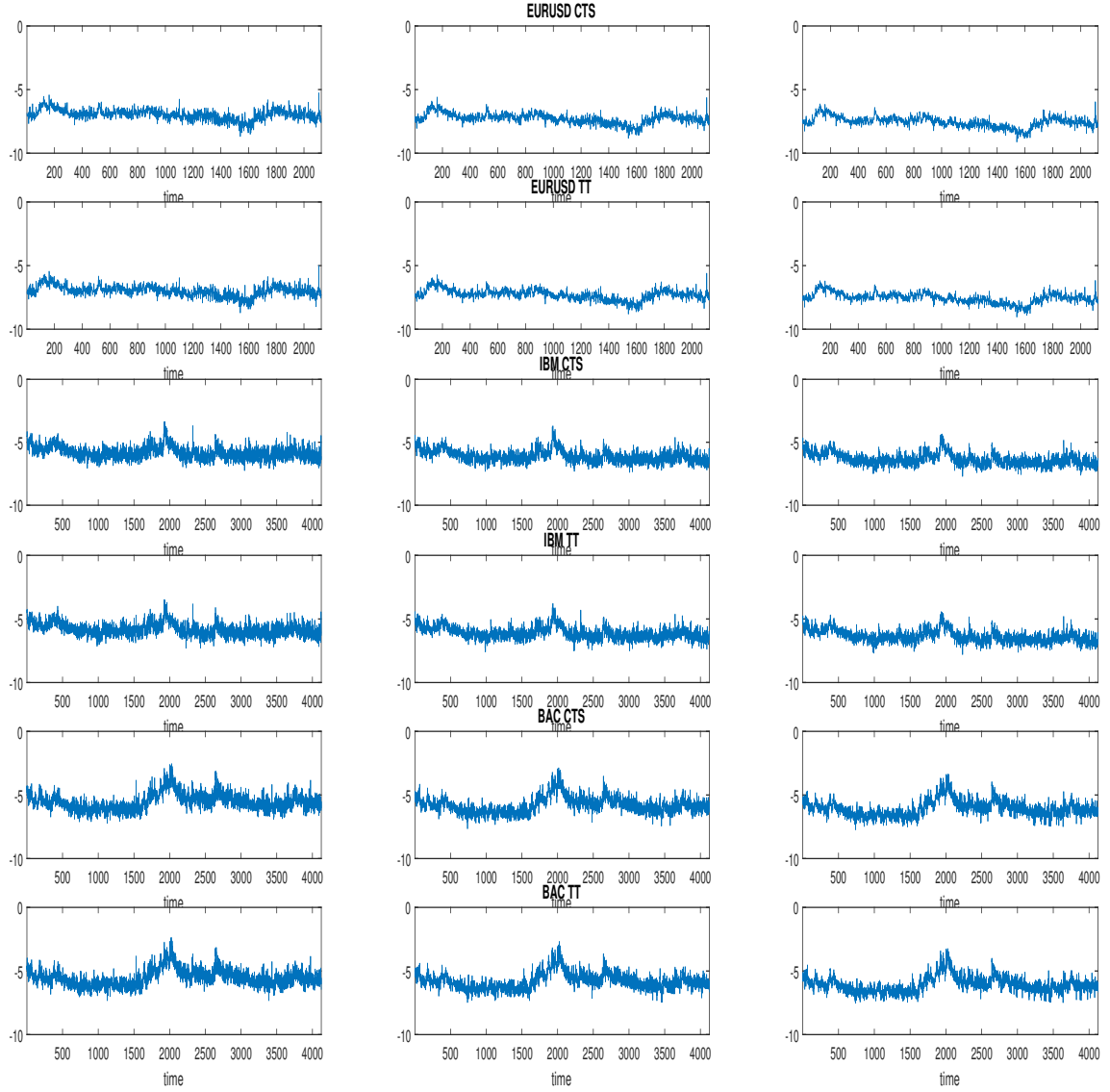
Figure C.1: Line graph of the log-transformation of the negative estimates of daily quantiles, \hat{q}_{p,d} , computed from scaling up estimates of intraday quantiles estimated from data sampled in TTS and CTS (use the DMA estimator of Hurst coefficient and the frequency of 5 minute to sample the data). The first column corresponds to p = 1\% , the second column corresponds to p = 2.5\% and the third column corresponds to p = 5\% .
