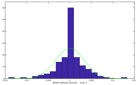
Figure 7: Histogram of residual series e(k) showing its non-normal distribution.
