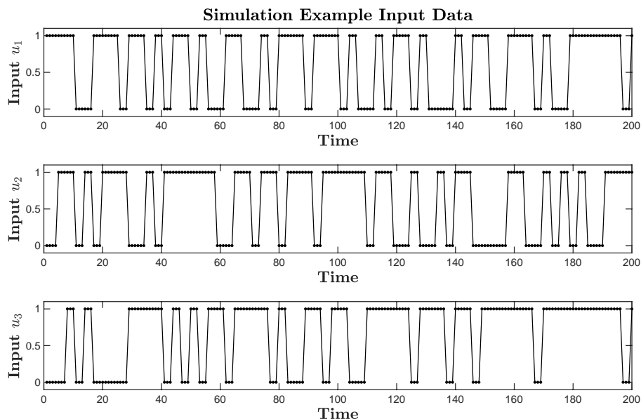
Figure 1: Inputs for the first simulated data example.
