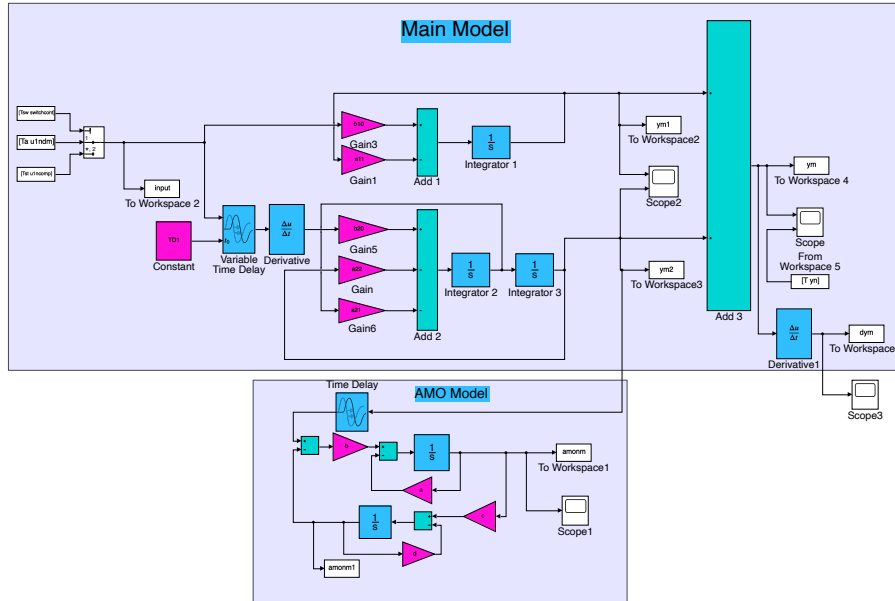
Figure 10: The Simulink diagram of a DBM model based on (7), as used in Young (2025), is shown the top, with a connected diagram for an AMO model below it.
